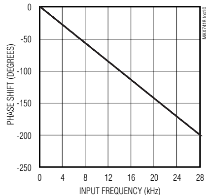
MAX7419/MAX7423 PHASE RESPONSE (BESSEL)
