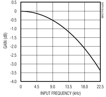
MAX7419/MAX7423 PASSBAND FREQUENCY RESPONSE (BESSEL)
